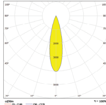
ArcSource Outdoor 48MC INT - 26°
