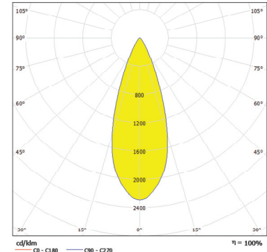
ArcSource Outdoor 48MC INT - 36°
