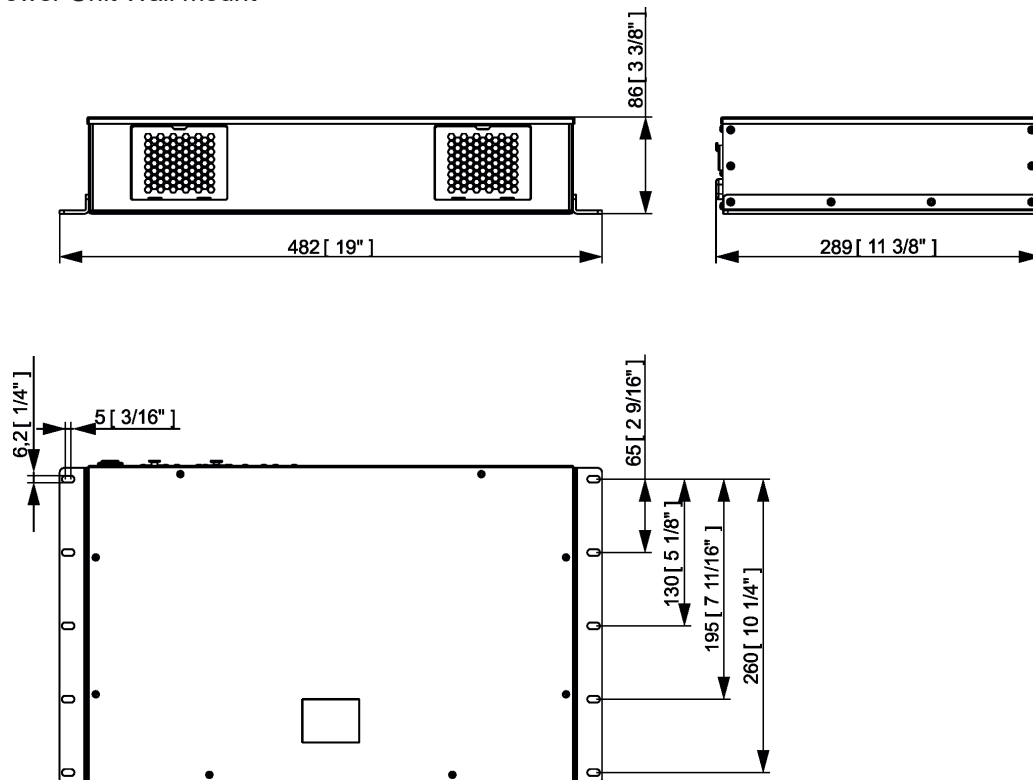
ArcPower Unit Wall mount
