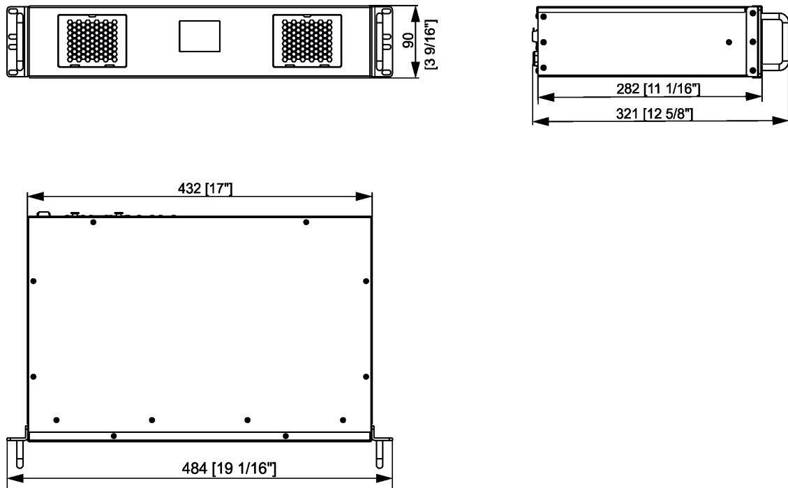
ArcPower Unit Rack Mount
