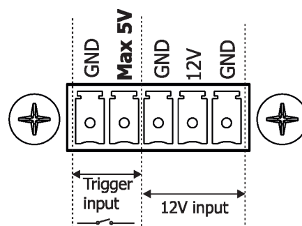
Trigger input and 12V output
