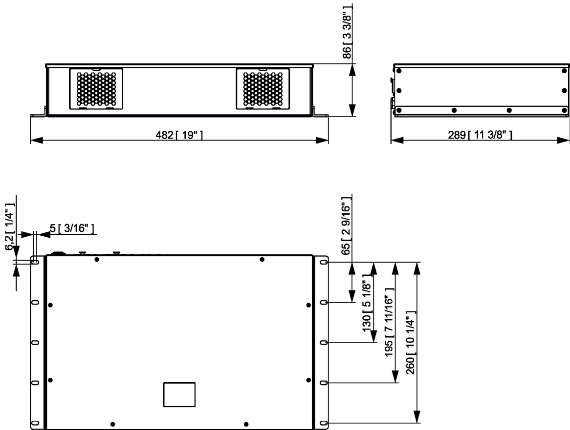
ArcPower Unit Pixel Rack Mount
