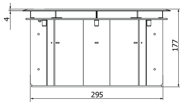
Installation sleeve
