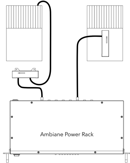
Connection of luminaire's power supply and Ambiane Power Rack.
