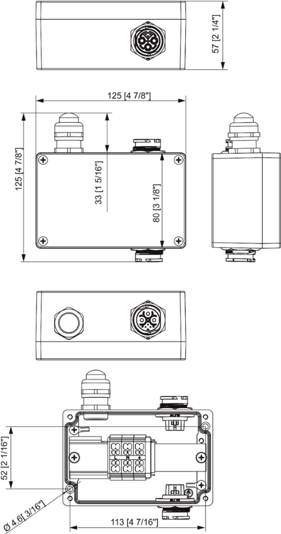
Booster box
