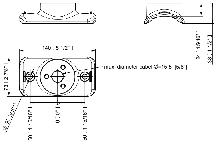
Pole Adaptor (Ø 102mm, Yoke for pole Adaptor Required / PA)
