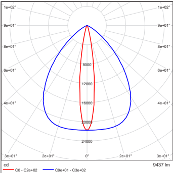
Calumma XL SC RGBW 6500K 15x90dg
