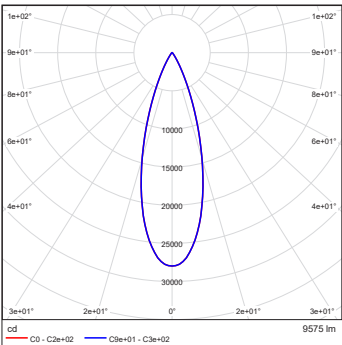
Calumma XL SC RGBW 6500K 30dg
