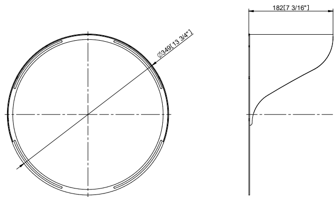
Floor Stand
