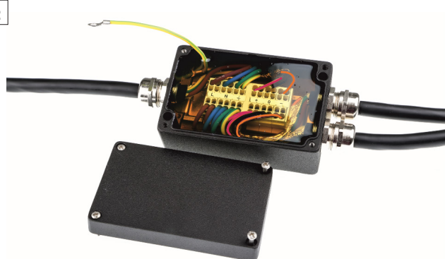
Prepared Junction Box and resin bag.
