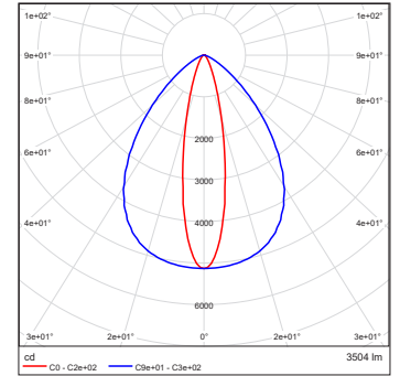
Eminere Inground 4 MC RGBCW Anti-Skid Glass 20dg x 90dg
