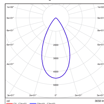
Eminere Inground 4 MC RGBCW Clear Glass 50dq
