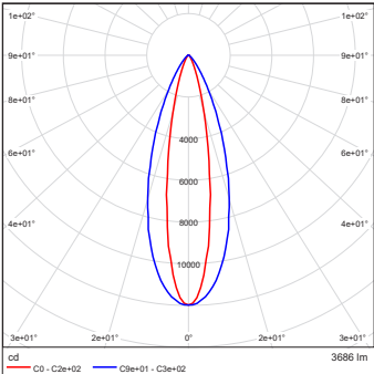
Eminere Inground 4 MC RGBCW Anti-Skid Glass 20dg x 35dg
