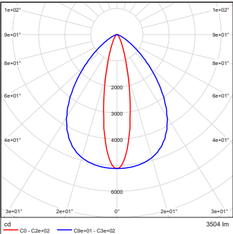
Eminere Inground 4 MC RGBCW Anti-Skid Glass 20dg x 90dg
