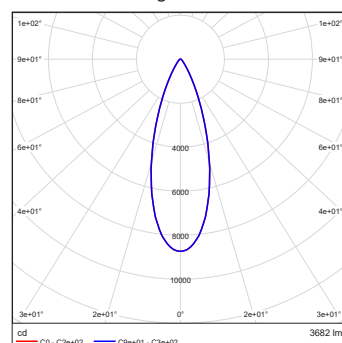
Eminere Inground 4 MC RGBCW Clear Glass 30dq
