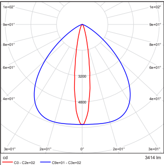
Eminere Inground 4 MC RGBCW Clear Glass 15dg x 90dg
