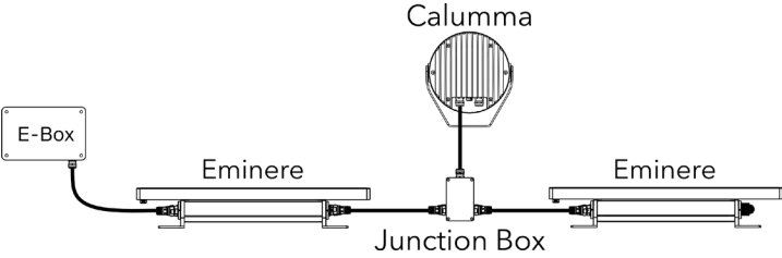
Cable Connection – EU colour coding
