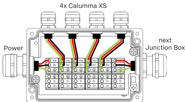
Junction Box
