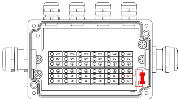
Junction Box
