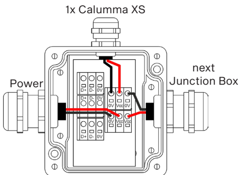
Junction Box
