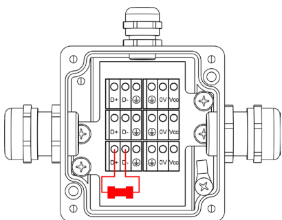
Junction Box
