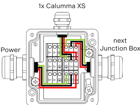
Junction Box
