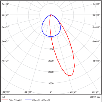
Eminere Inground 4 MC RGBCW Anti-Skid Glass Wide WallWasher
